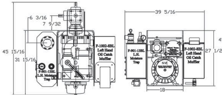
367 CCW "Max Pack" Assembly F-1000-2MTCCW
