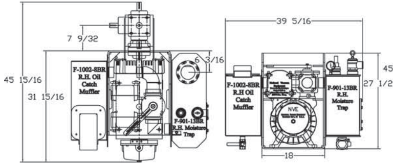
367 CCW "Max Pack" Assembly F-1000-2MTCCW
