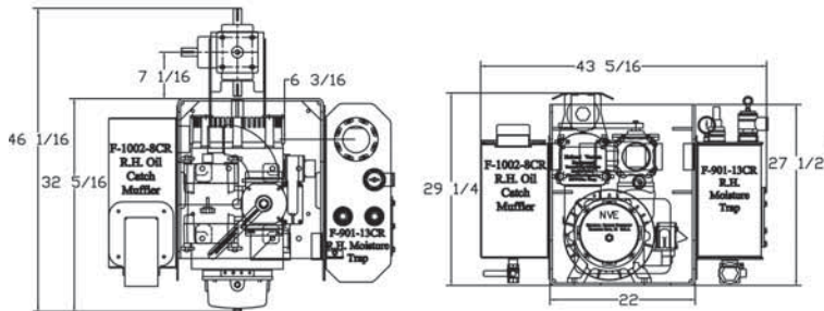
506 CCW "Max Pack" Assembly F-1000-3MTCCW
