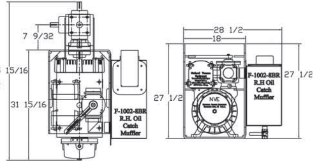
367 CCW "Muffler Pack" Assembly F-1000-2MCCW
