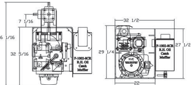
506 CCW "Muffler Pack" Assembly F-1000-3MCCW
