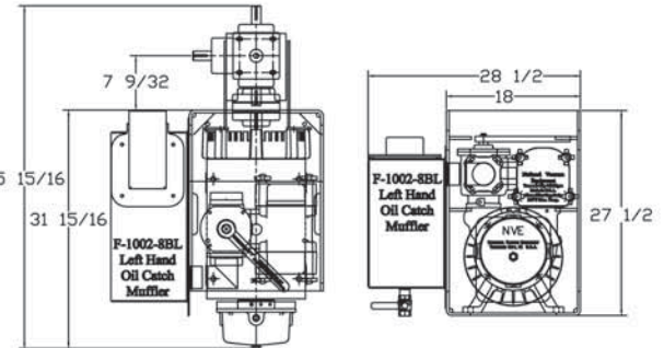
367 CCW "Muffler Pack" Assembly F-1000-2MCCW
