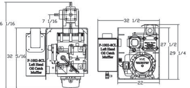
506 CCW "Muffler Pack" Assembly F-1000-3MCCW
