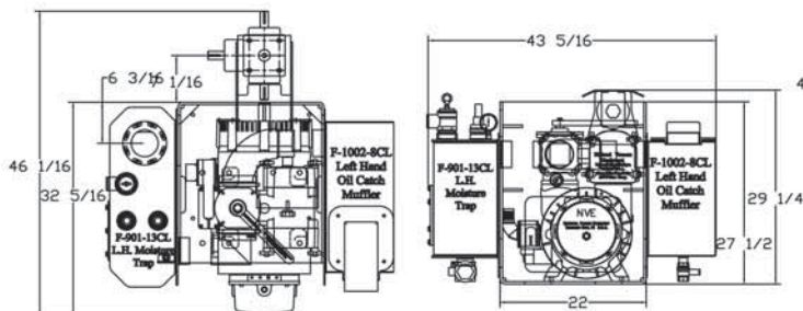
506 CCW "Max Pack" Assembly F-1000-3MTCCW
