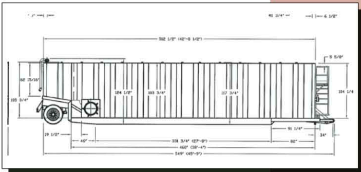
Tank Dimensions
