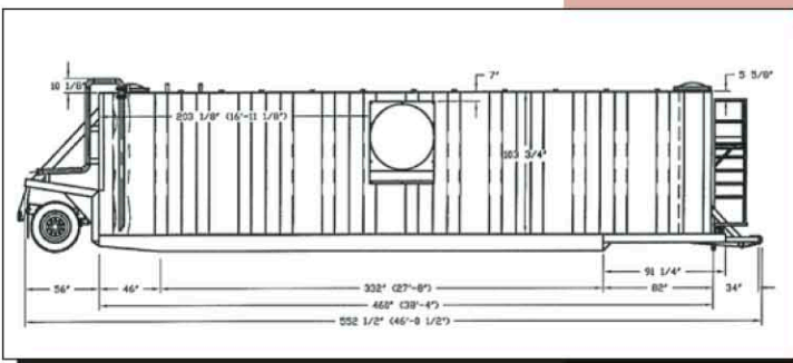
Tank Dimensions
