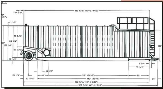
Tank Dimensions
