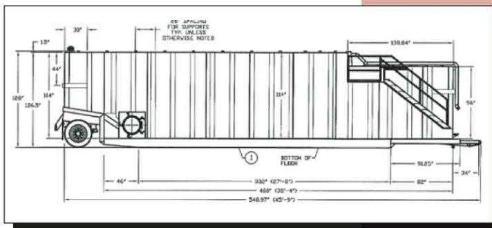
Tank Dimensions
